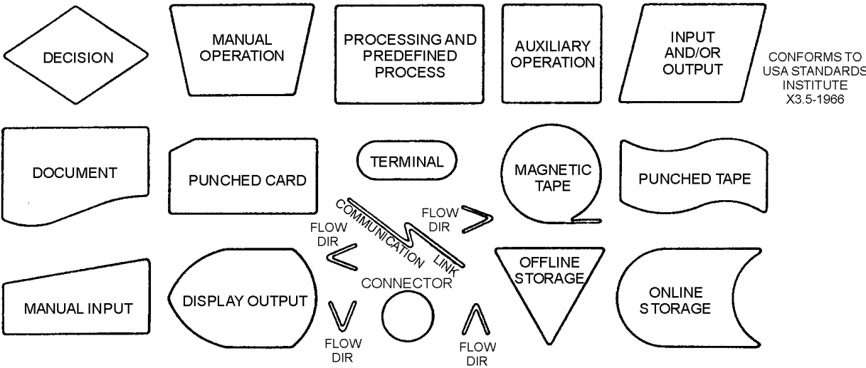
Figure 3-4.—Flowchart template.
