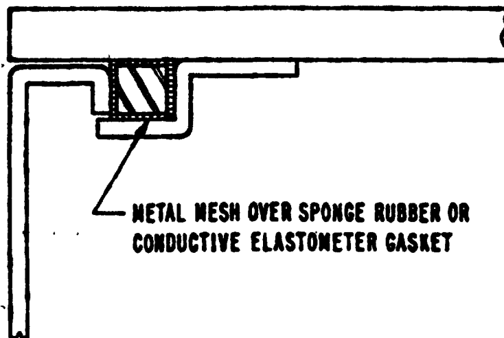
FIGURE 48. RAIN TIGHT CONDUCTIVE GASKET SEAL
