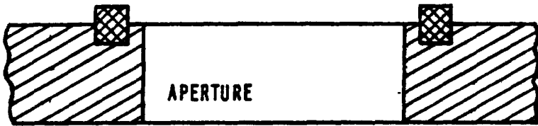
A. HELD IN PLACE IN SLOT BY SIDE-WALL FRICTION
