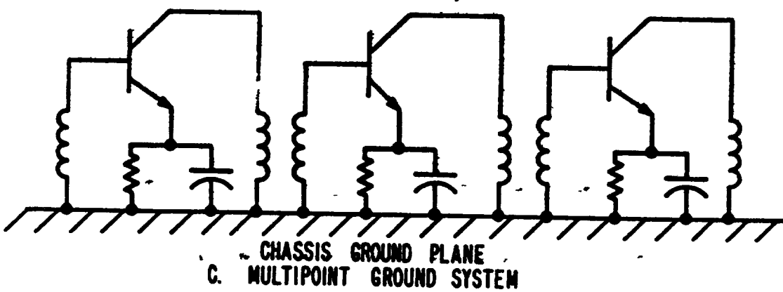
FIGURE 1. GROUND SYSTEMS
