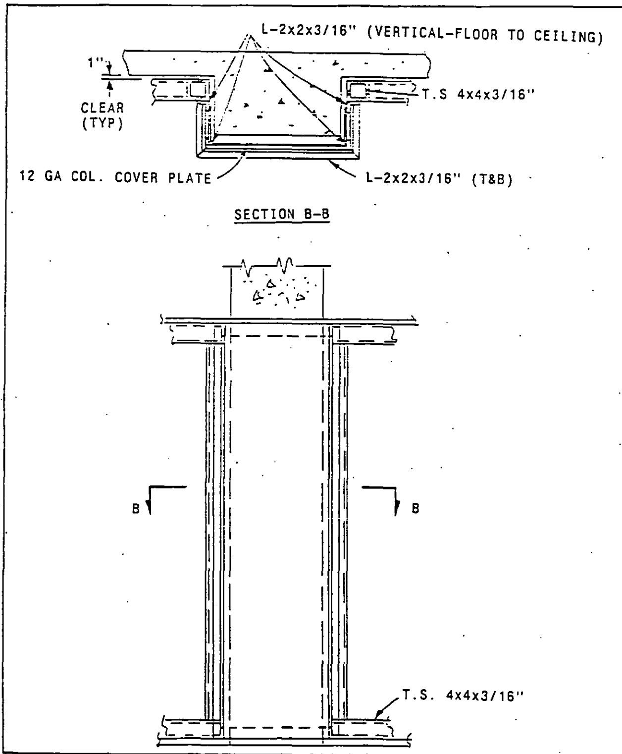
Figure 9 RF Shielding, Exterior Concrete Column
