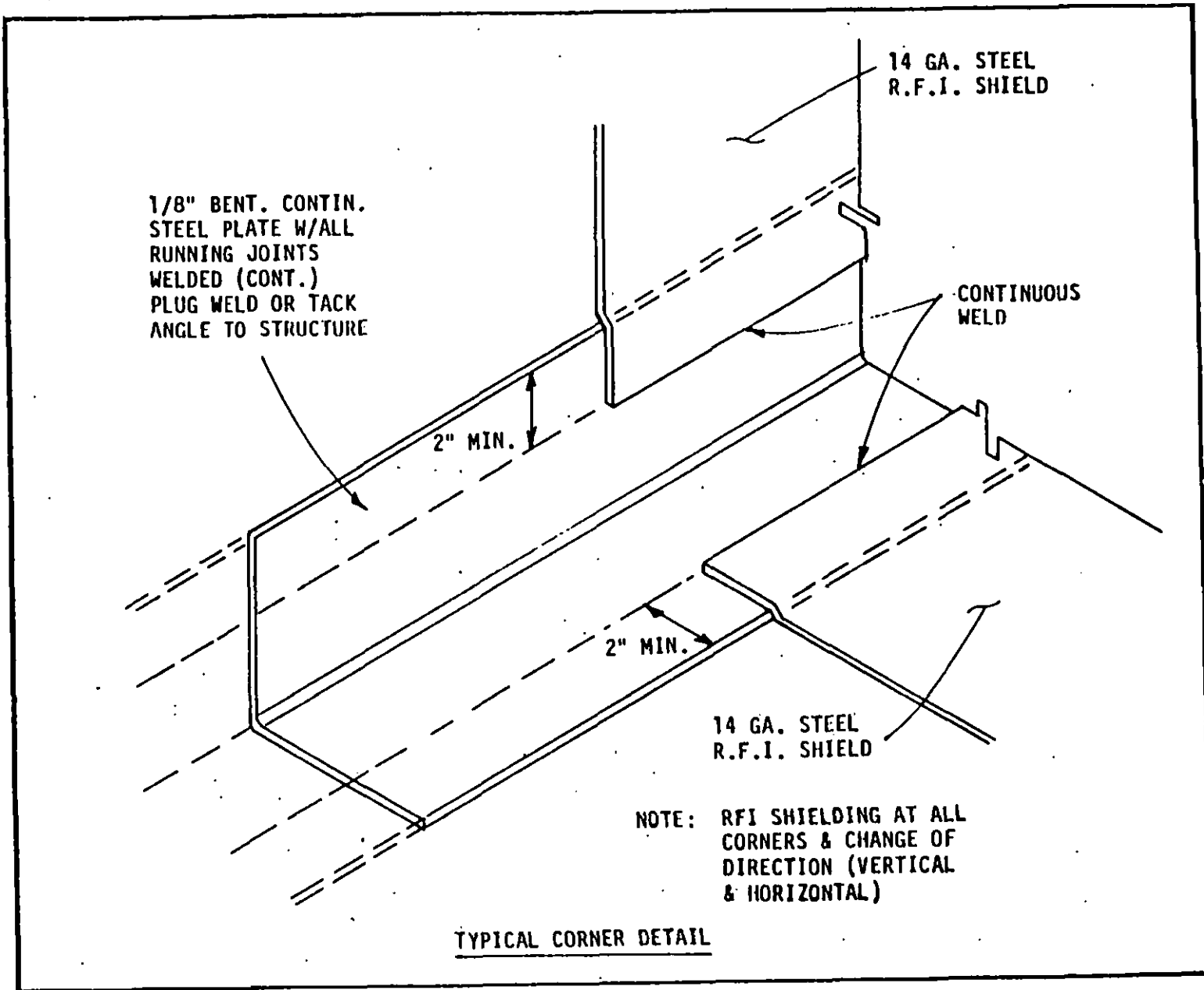
Figure 23 RF Shielding of Floor-wall Intersection With Overlap Seams
