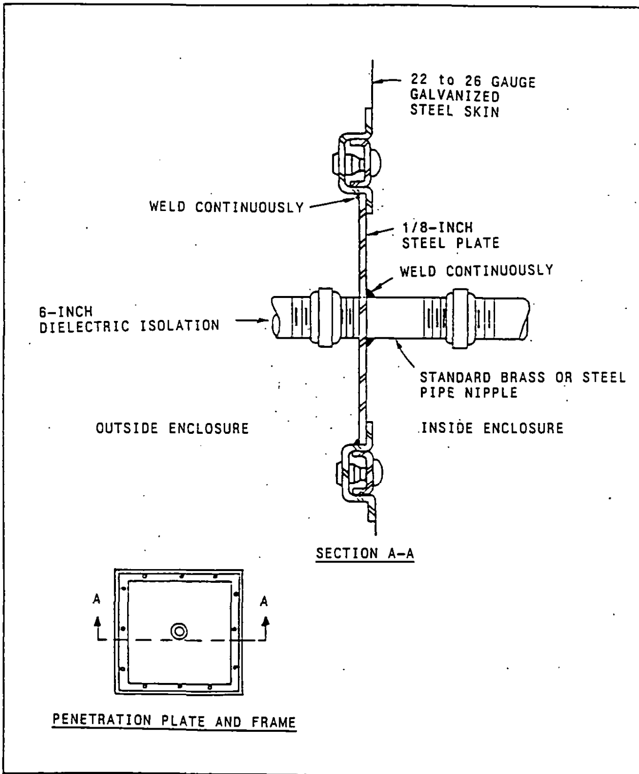
Figure 4 Single Skin Bolted Enclosure Penetration Panel
