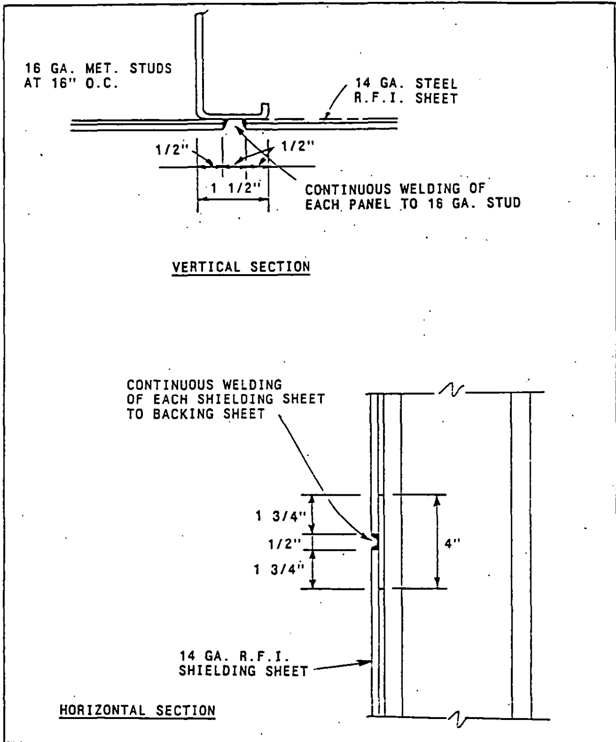
Figure 17 RF Wall Shielding, Seam Detail
