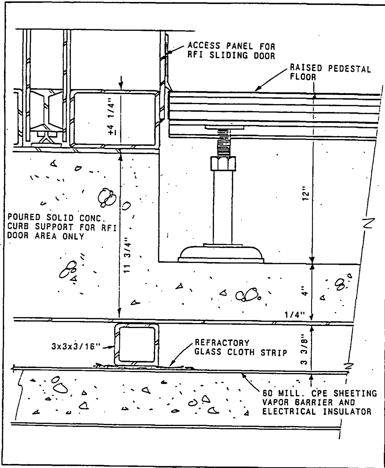
Figure 20 RF Shielding, Sliding Door Frame Section
