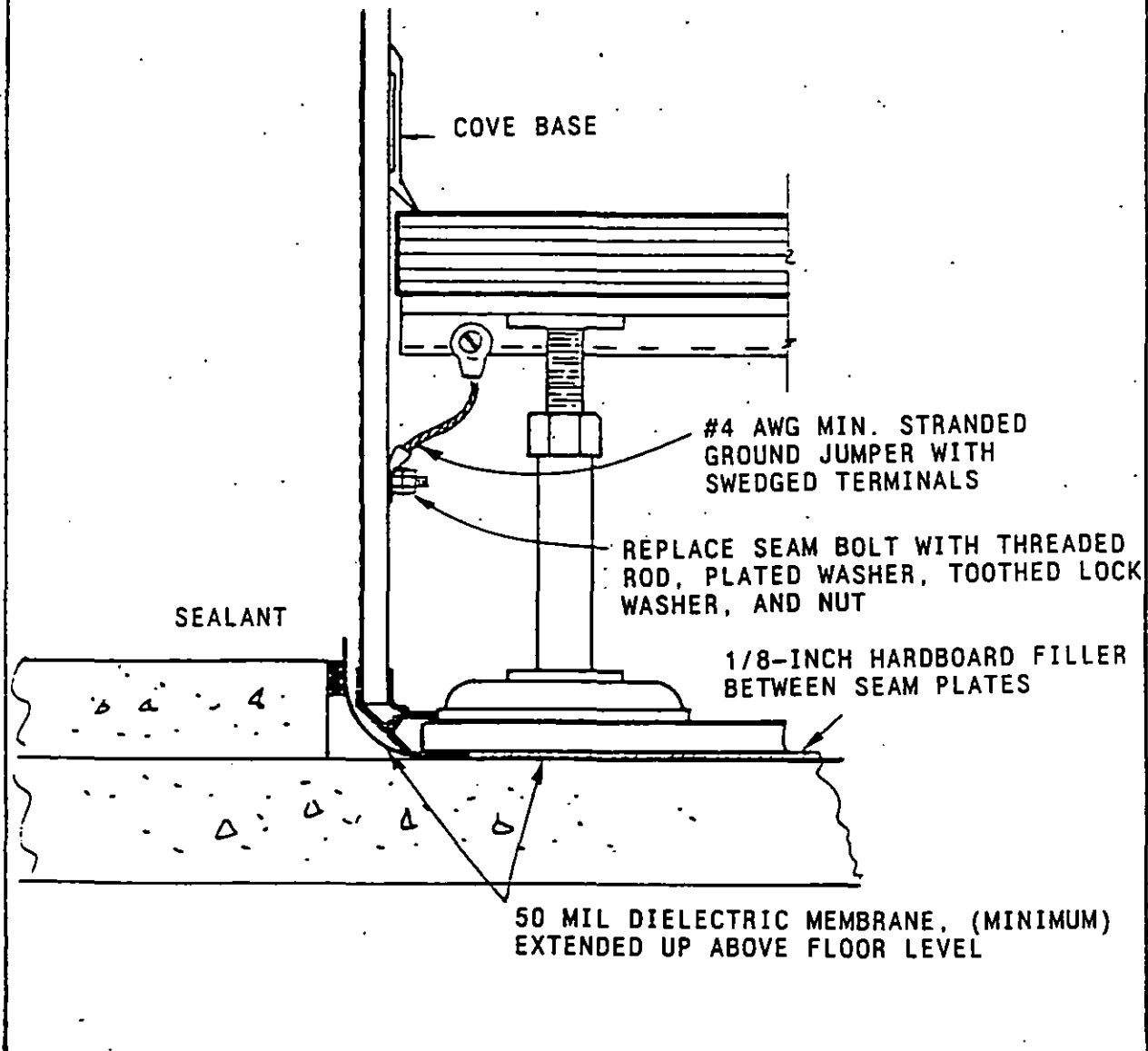
Figure 12 High Frequency Grounding, Using Raised Flooring as an Equipotential Plane
