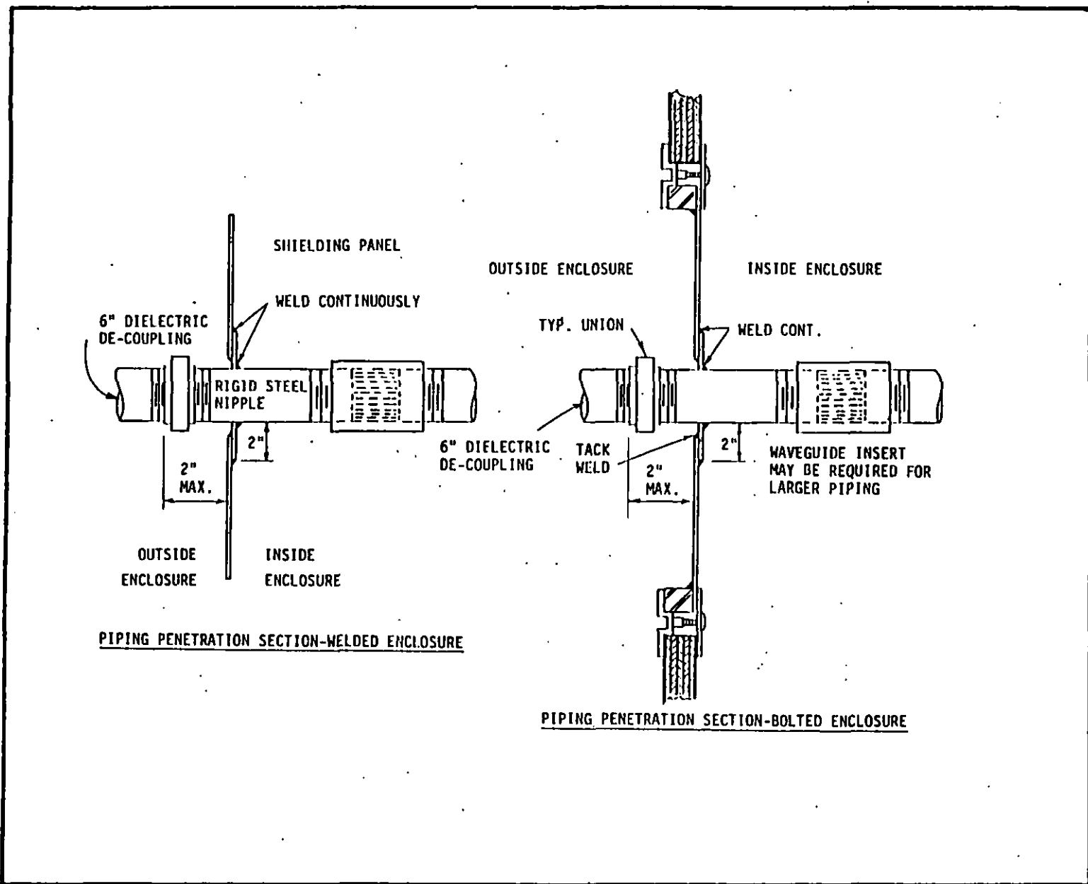
Figure 3 Typical TEMPST Pipe penetration, Bolted and Welded Enclosure
