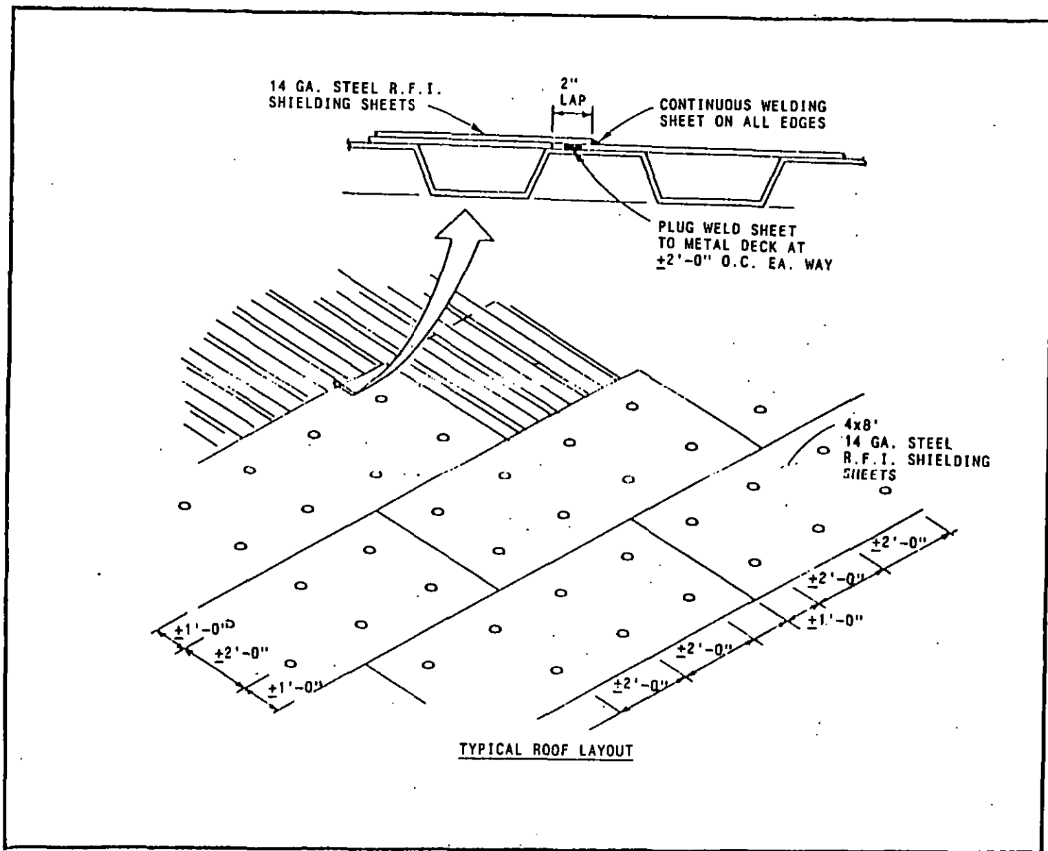
Figure 25 RF Shielding, Roof Layout With Metal Decking
