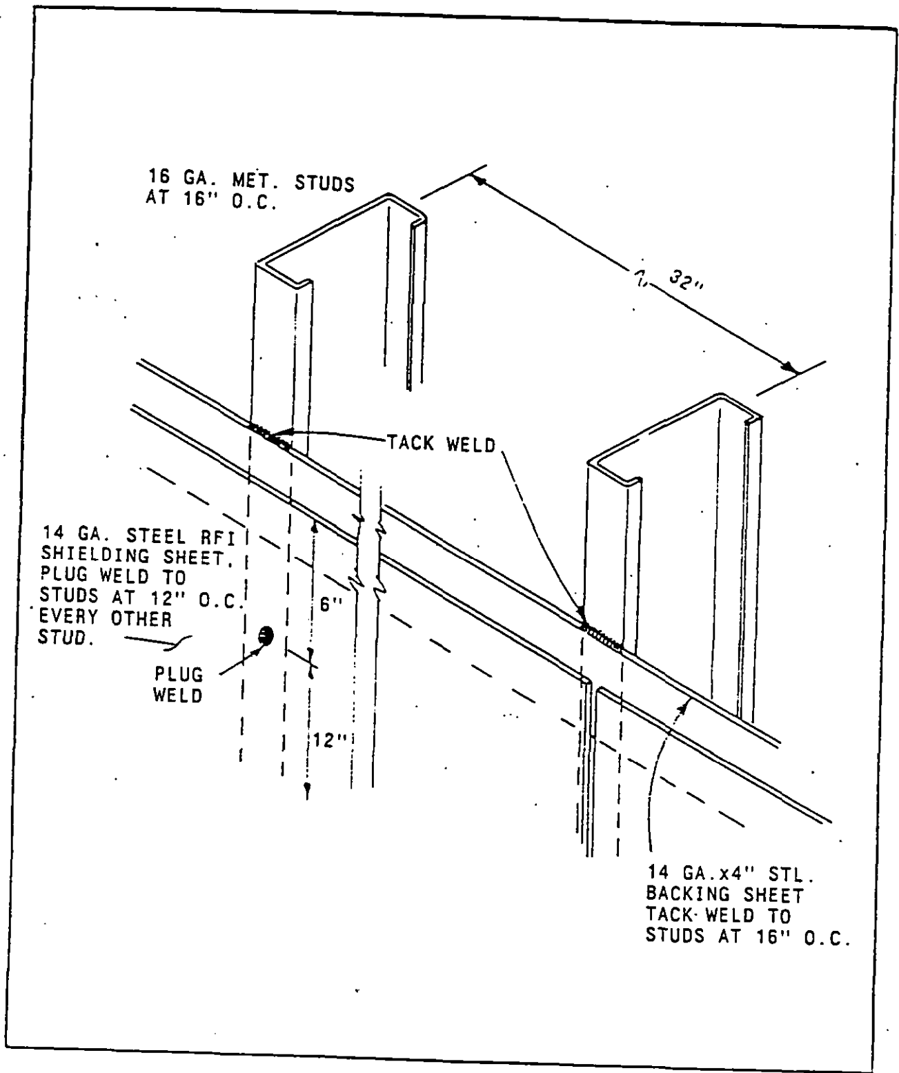
Figure 16 Welded RF Shielding of Wall Section
